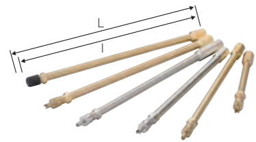
*Truck & Bus Metal Extensions
