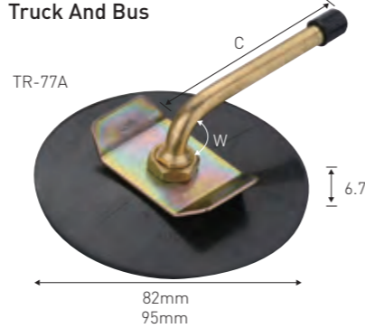
*TRJ650 Series Large Bore Tubeless Valves-Swivel Type
