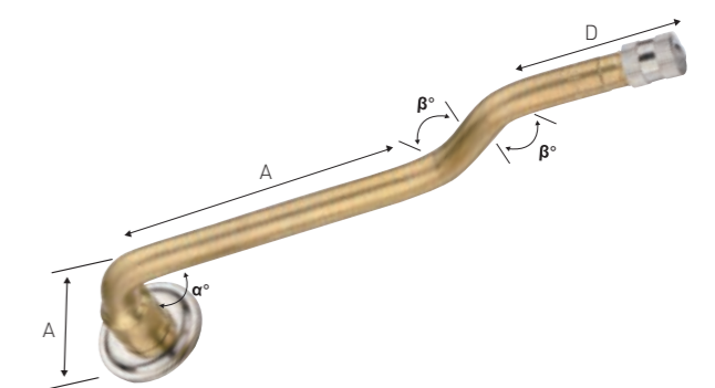
*Triple Bend Type
