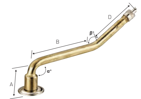
*Double Bend Type
